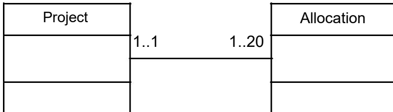
Figure 12.22 Association showing defined range of multiplicity
