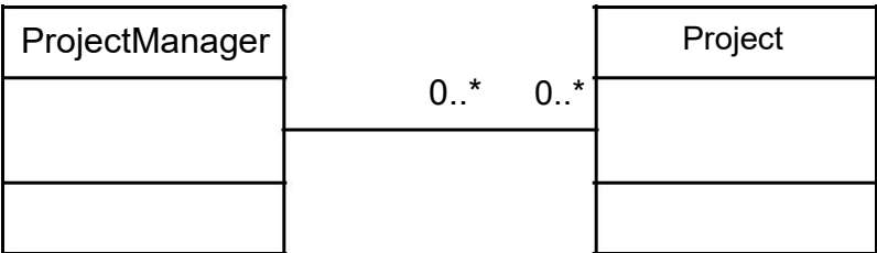
Figure 12.23 Association with many:many multiplicity
