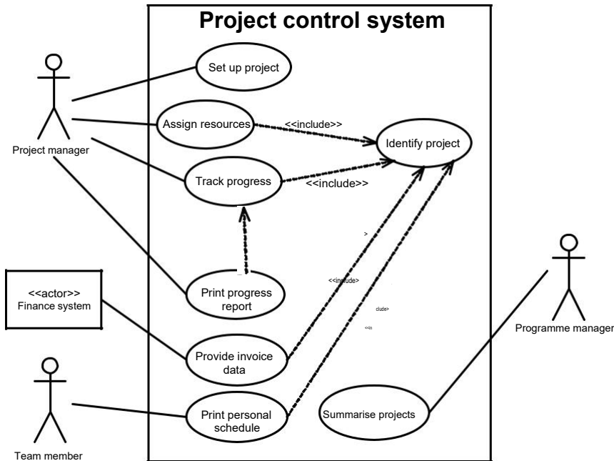
Figure 12.4 Use case diagram showing <<include>> and <<extend>>
