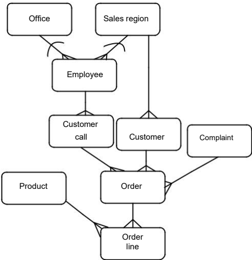
Figure 12.15 Entity relationship diagram for a sales system
