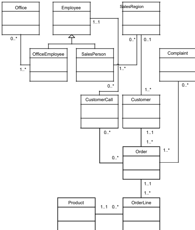
Figure 12.26 Class model for a sales system
