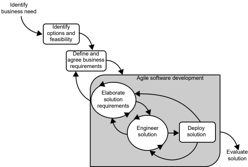
Figure 13.7 Generic Agile model
