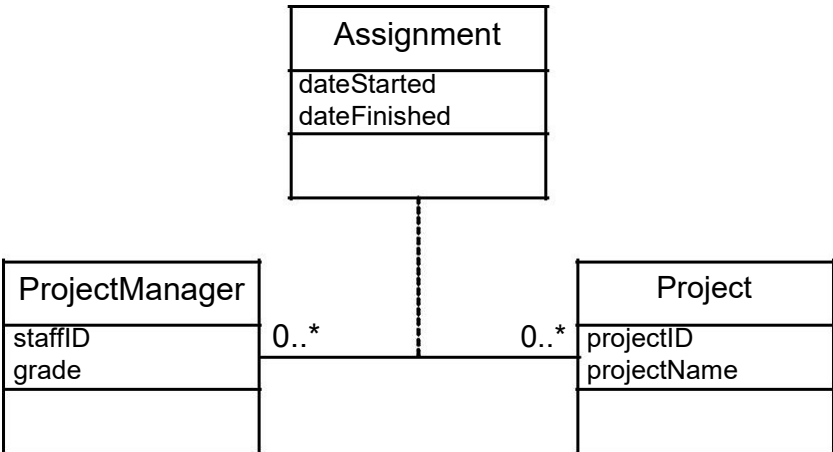
Figure 12.24 An association class
