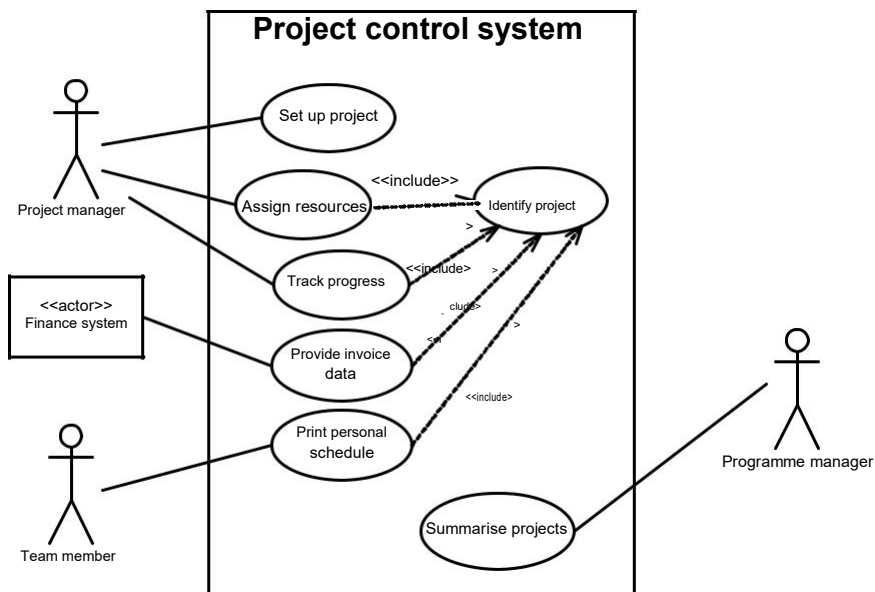
Figure 12.3 Use case diagram showing <<include>>
