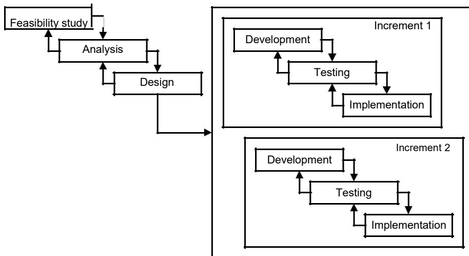
Figure 13.6 Incremental lifecycle
