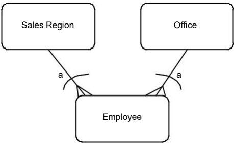
Figure 12.14 Exclusive relationships
