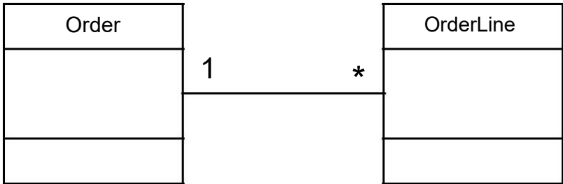
Figure 12.19 Association showing one-to-many multiplicity
