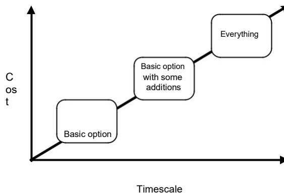
Figure 9.3 Incremental options
