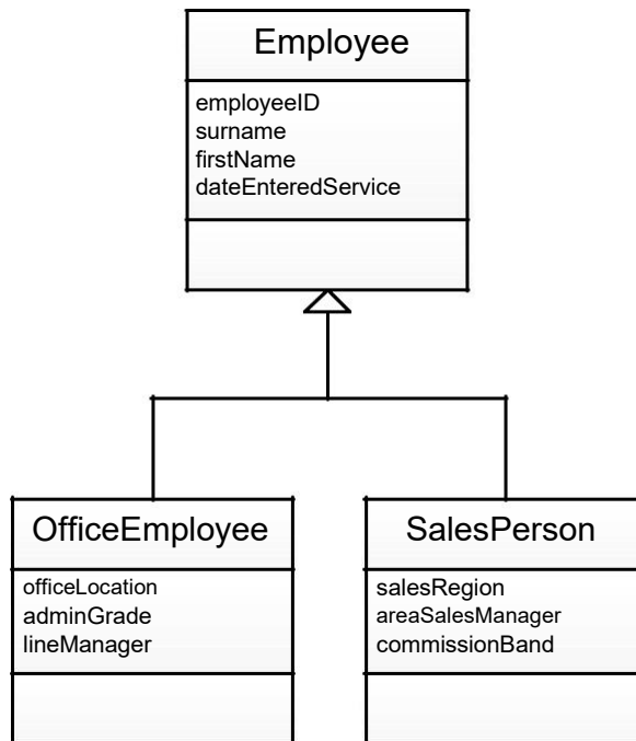
Figure 12.25 Generalisation structure
