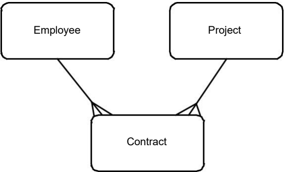
Figure 12.12 Resolved many-to-many relationship
