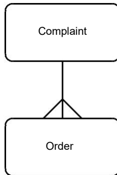
Figure 12.10 Optional parent entity with mandatory child entity
