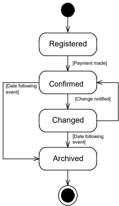
Figure 14.4 Example state chart
