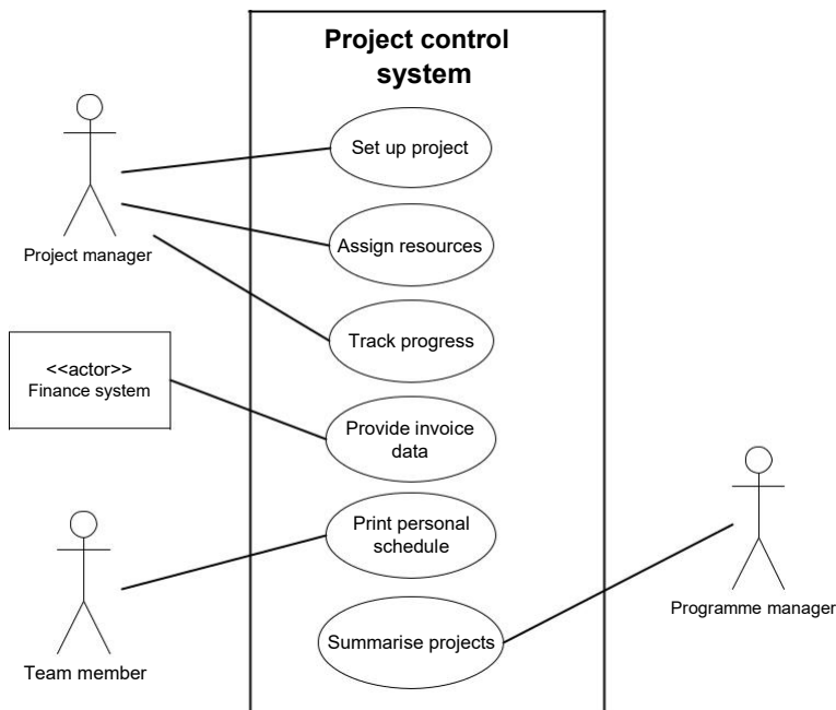
Figure 12.2 System use case diagram for a project control system
