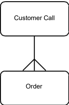
Figure 12.8 Fully optional one-to-many relationship
