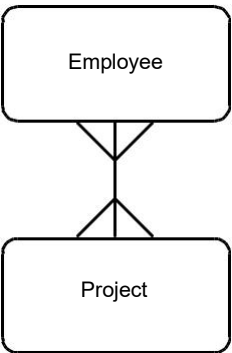
Figure 12.11 Many-to-many relationship
