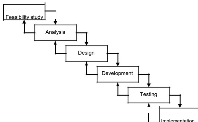
Figure 13.3 The waterfall lifecycle
