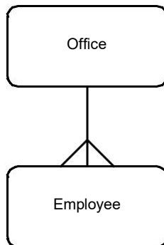
Figure 12.5 One-to-many relationship between two entities
