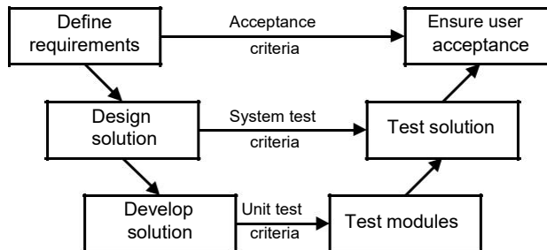
Figure 13.4 The 'V' model
